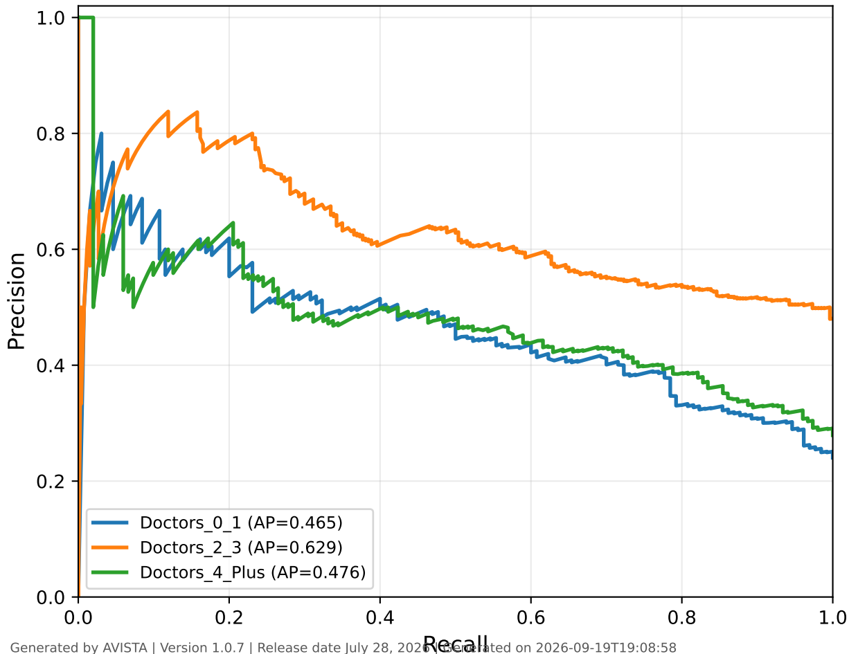
Precision-Recall Curve - Logistic Regression - Train
