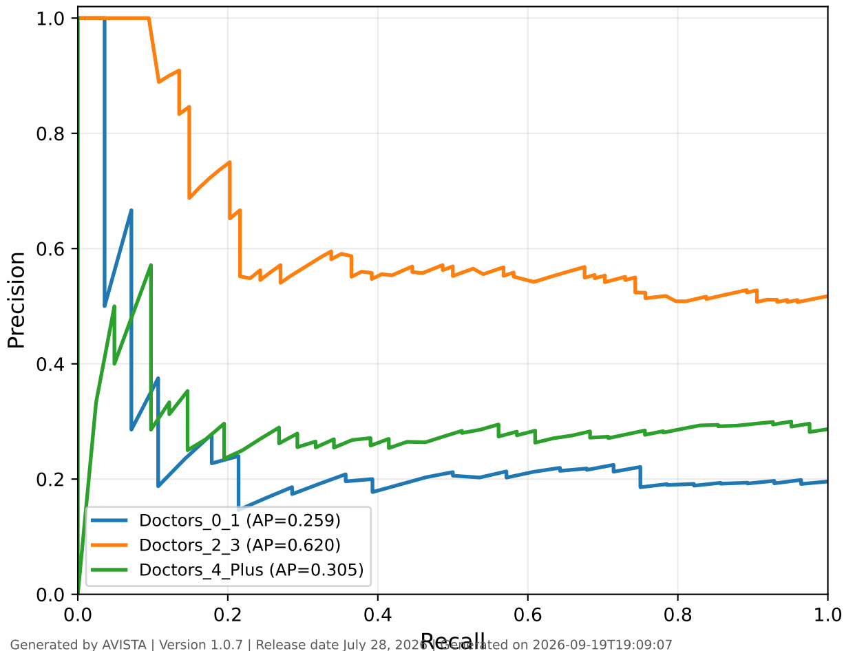
Precision-Recall Curve - Random Forest - Test
