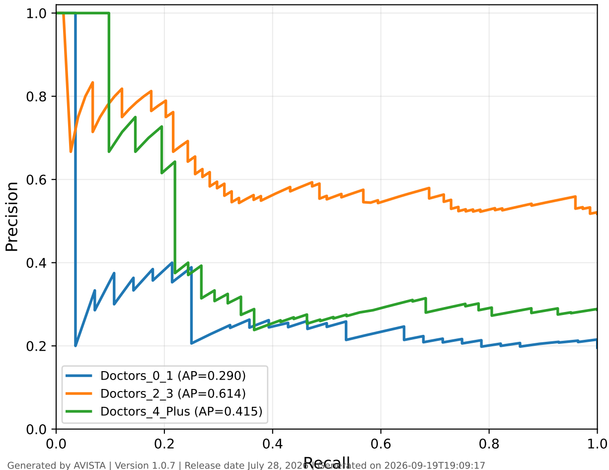
Precision-Recall Curve - XGBoost - Test
