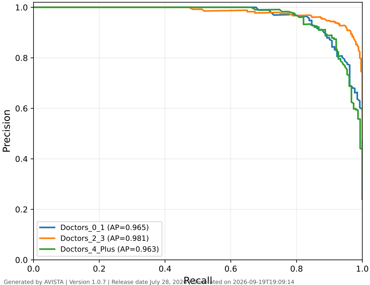
Precision-Recall Curve - XGBoost - Train
