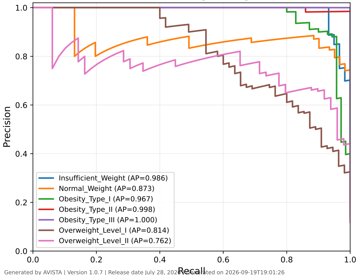
Precision-Recall Curve - Logistic Regression - Test
