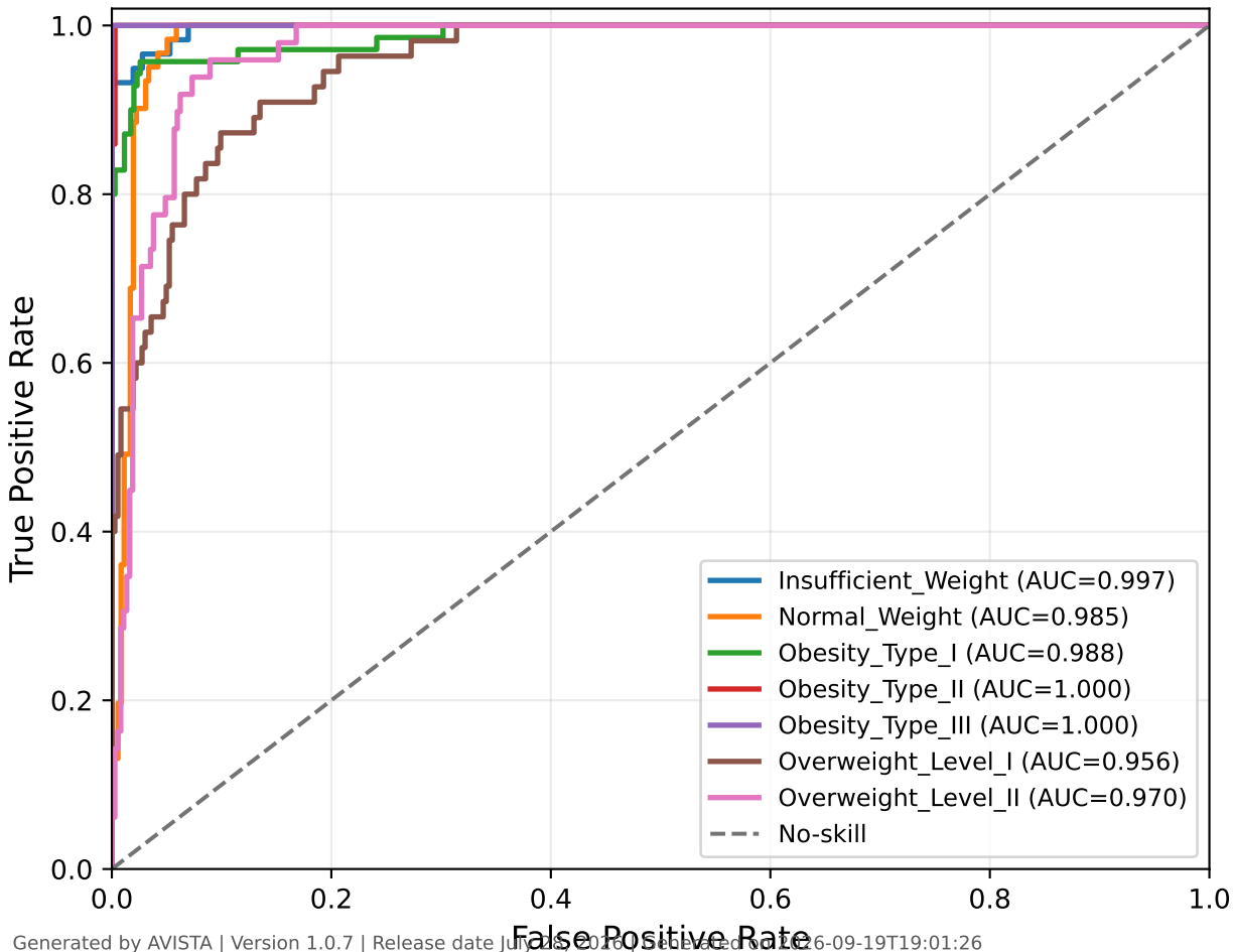
ROC Curve - Logistic Regression - Test
