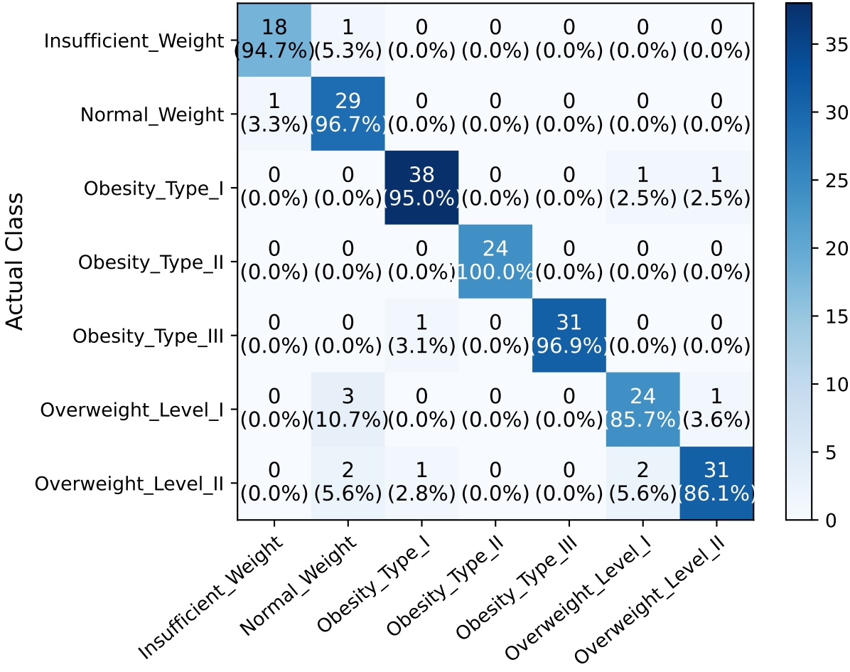
Confusion Matrix - Random Forest - Validation
