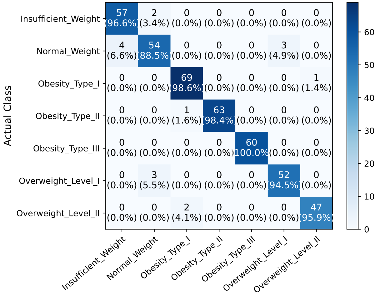
Confusion Matrix - XGBoost - Test
