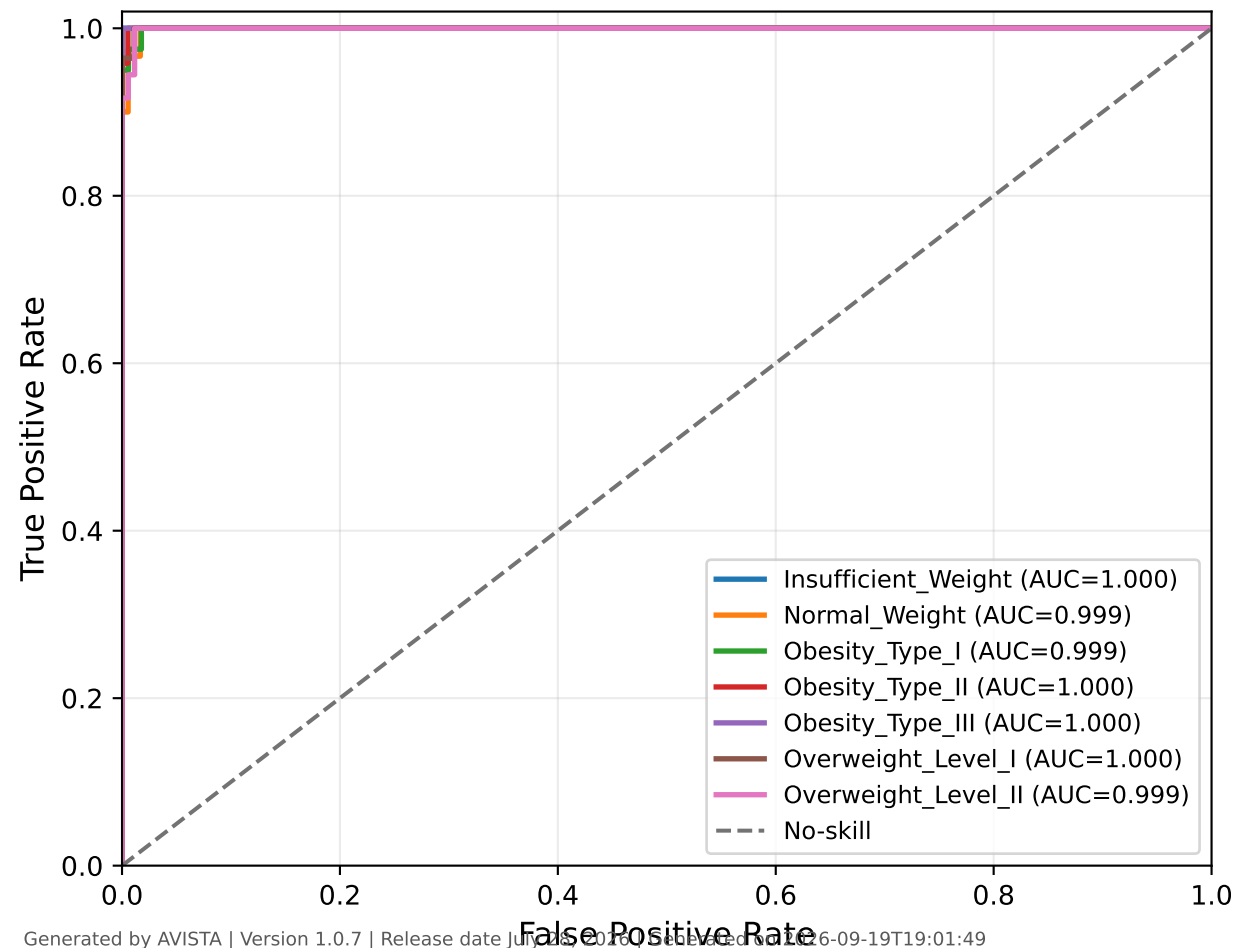
ROC Curve - XGBoost - Validation
