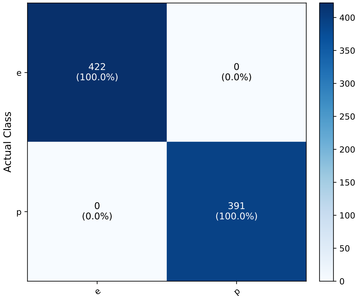
Confusion Matrix - XGBoost - Validation
