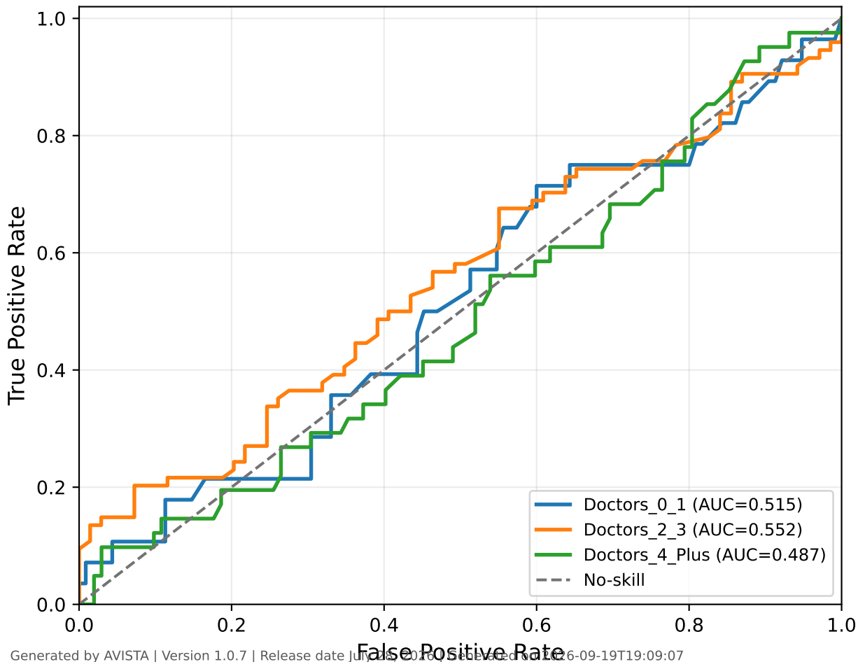
ROC Curve - Random Forest - Test
