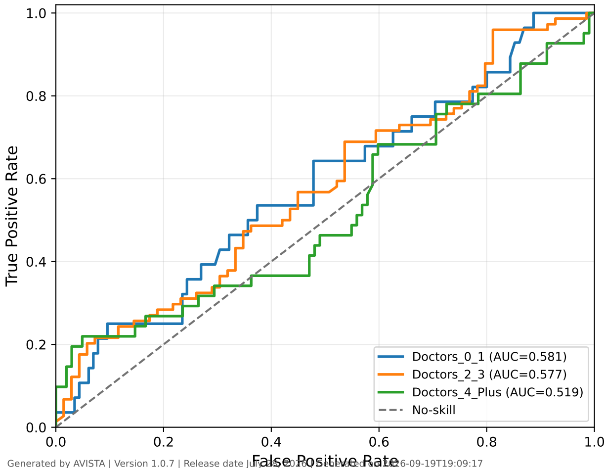
ROC Curve - XGBoost - Test
