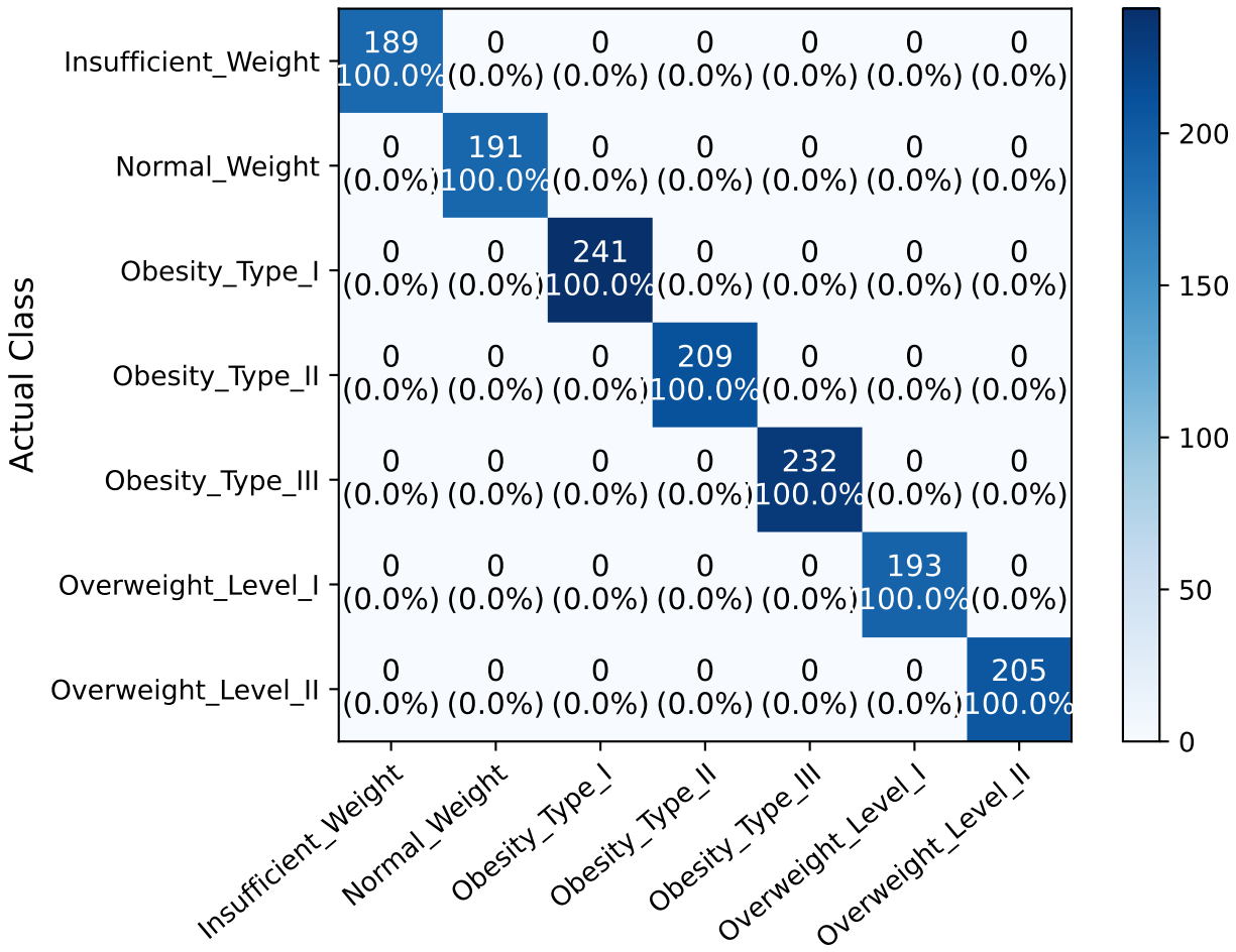
Confusion Matrix - Random Forest - Train
