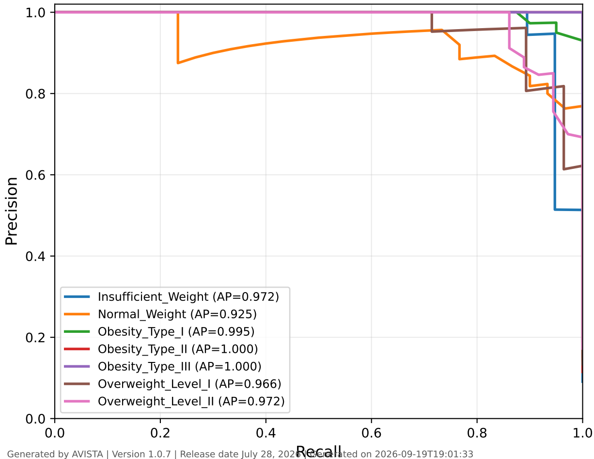
Precision-Recall Curve - Random Forest - Validation
