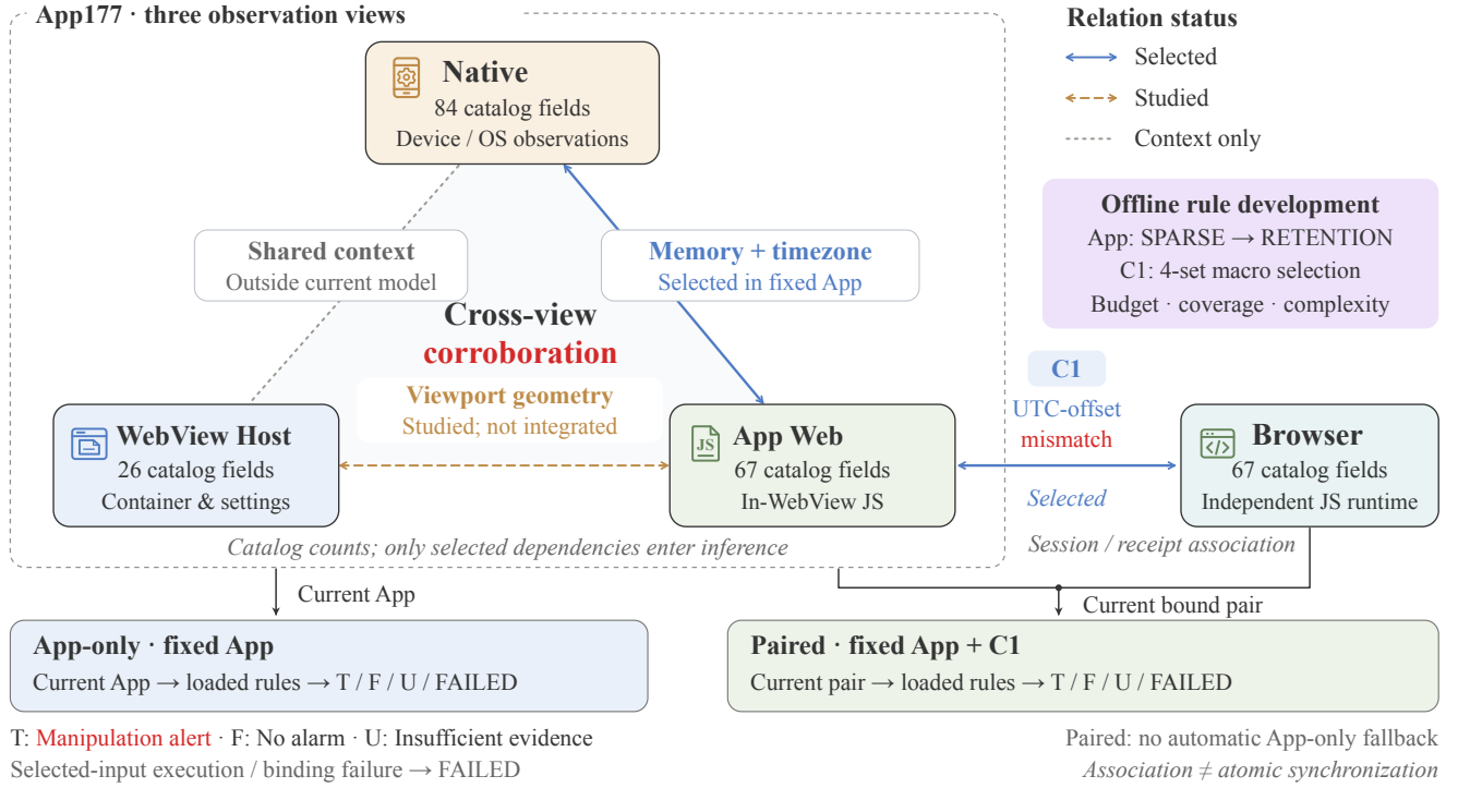
Figure 1: HybridGuard as a triangle of complementary observation views. Native, WebView Host, and App Web provide device/system, container/settings, and webpage-runtime observations. Solid blue edges denote relations selected in the retained models: Native–App Web memory and timezone relations, and the App Web–independent Browser numeric UTC-offset condition C1. The dashed ochre edge denotes separately studied Host geometry that is not integrated; the arrowless dotted gray edge denotes only shared Native–Host context outside the current App rule pool. Arrowed comparison edges identify the views being compared, not bidirectional rule execution or trusted ground truth. The App detector combines within-view rules with selected cross-view relations. Offline development applies App SPARSE selection and RETENTION, followed by constrained macro-detection selection over four cross-endpoint sets. Separate App-only and paired interfaces load fixed models and read only current inputs. T denotes a manipulation alert, F no alarm, and U insufficient evidence; execution or binding failures in selected inputs take precedence as FAILED. Paired inference has no automatic App-only fallback. Field counts describe catalogs, binding IDs are not detection features, and association does not imply atomic synchronization.
