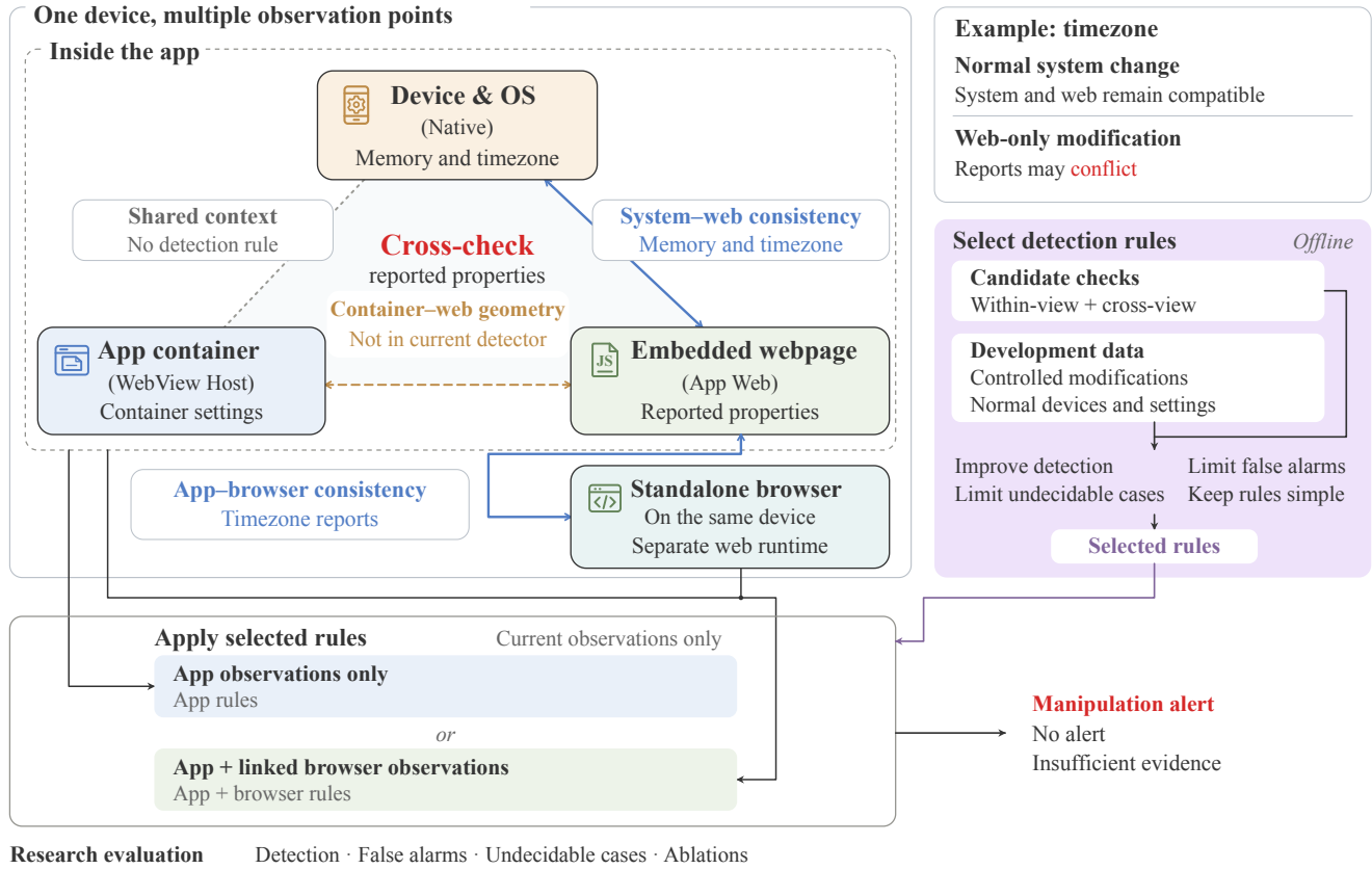
Figure 1: HybridGuard checks device-fingerprint reports for possible manipulation using complementary observations from the same device. Within-view and cross-view checks are evaluated on controlled modifications and normal operation to select compact detection rules under false-alarm and decision-coverage constraints. The selected detectors process current App observations alone or linked App-browser observations and return a manipulation alert, no alert, or insufficient evidence. The inset illustrates why changing a system setting need not have the same cross-view effect as modifying only a webpage’s report. Solid comparison edges indicate relations used in the detectors; Host-web geometry remains a separate study, and the dotted Native-Host link denotes context only. No observation point is trusted ground truth. No alert does not establish safety. Execution failures are recorded separately.
