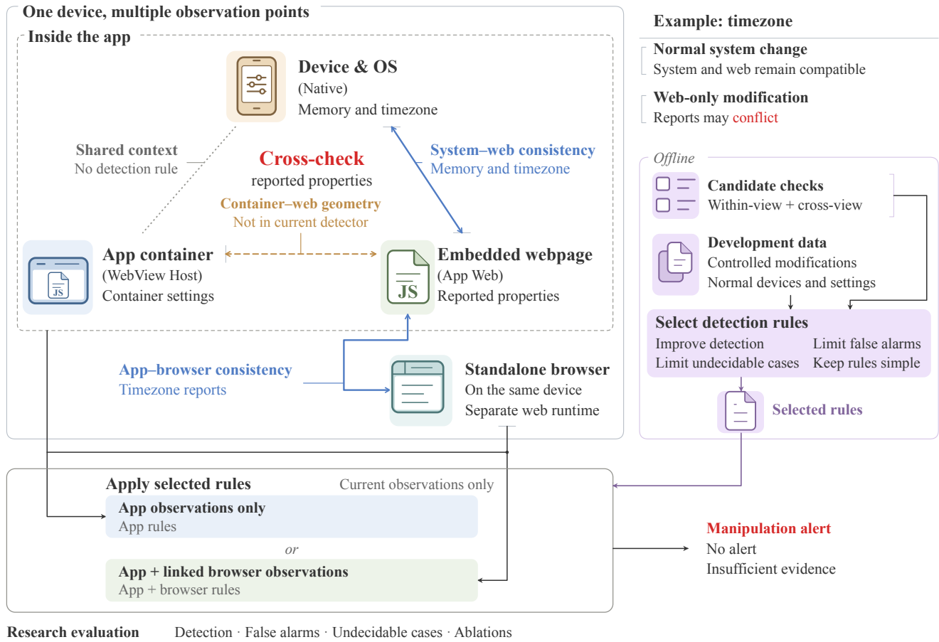
Figure 1: HybridGuard checks device-fingerprint reports for possible manipulation using complementary observations from the same device. Within-view and cross-view checks are evaluated on controlled modifications and normal operation to select compact detection rules under false-alarm and decision-coverage constraints. The selected detectors process current App observations alone or linked App-browser observations and return a manipulation alert, no alert, or insufficient evidence. The inset illustrates why changing a system setting need not have the same cross-view effect as modifying only a webpage’s report. Solid comparison edges indicate relations used in the detectors; Host-web geometry remains a separate study, and the dotted Native-Host link denotes context only. No observation point is trusted ground truth. No alert does not establish safety. Execution failures are recorded separately.
