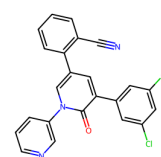
7L10, XEY (5.4)
