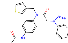
7GD4, R3O (5.79)
