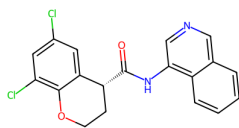
7GIN, QH1 (6.58)
