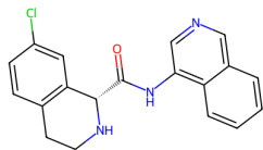
7CK6, QTL (5.95)
