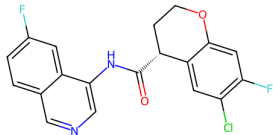
7CKB, QVG (6.5)
