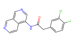
7GJL, QH6 (5.73)
