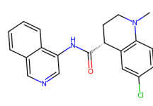
7GJ5, P4X (6.61)
