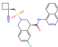
7GLT, RC9 (7.22)
