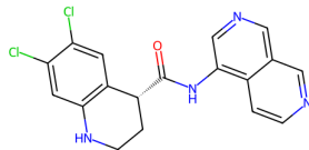
7CKD, QVU (5.98)
