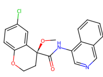
7GJ3, P46 (7.08)
