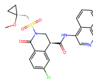
7GN5, RT9 (6.68)
