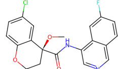
7CKN, QY1 (6.79)
