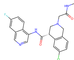
7CM4, RCQ (6.59)
