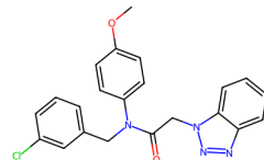
7GG7, OQX (5.94)
