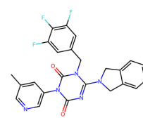
9LVR, A1L7P (5.84)
