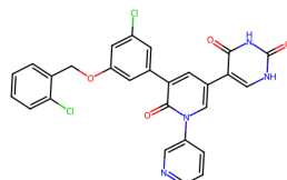
7L13, XF7 (7.74)
