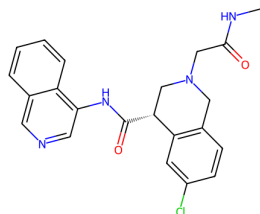
7CKV, R0F (7.1)
