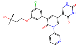
7MBZ, YTV (6.6)
