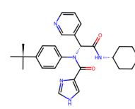
8YK1, X77 (5.55)
