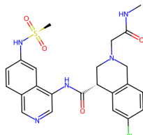
7CM1, RFR (6.54)
