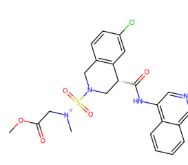
7GLI, R9I (6.94)
