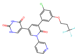
7M9I, YU4 (7.6)
