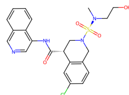
7GLX, RDX (6.92)
