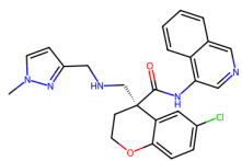
7GJF, QMX (6.1)
