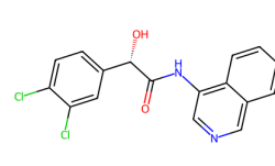
7GJ6, QH6 (5.7)
