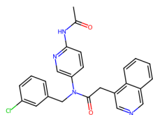
7GJ9, QL3 (6.17)
