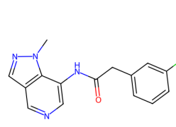
7CKY, R1U (5.83)
