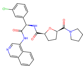
7GL0, R2X (6.34)
