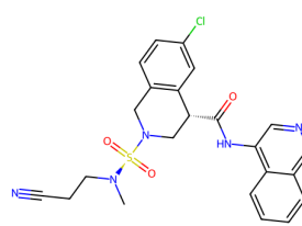
7GLM, RBM (7.07)
