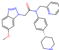
7GFJ, OD7 (4.41)
