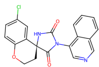
7GIX, P4R (6.16)
