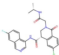
7GN2, RS6 (6.09)
