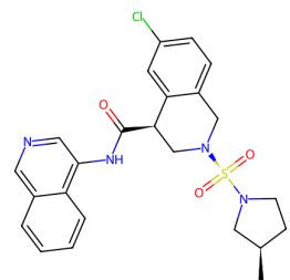
7CKS, QZL (7.29)
