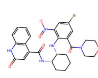
8Y44, A1D50 (6.7)
