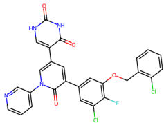
7MBP, Y5I (7.7)
