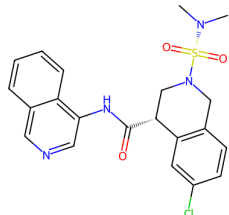
7CKR, QZC (6.85)
