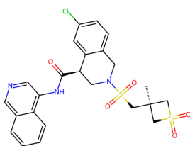
7GLJ, R9R (7.25)
