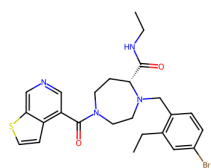
9HAK, A1I7I (7.8)
