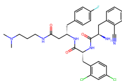
8UDW, WDK (7.7)
