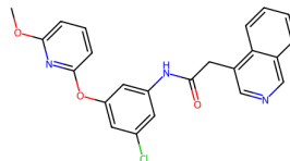
7GFE, O9O (5.42)
