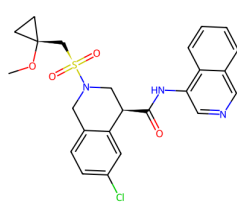
7GLK, R9Z (7.0)
