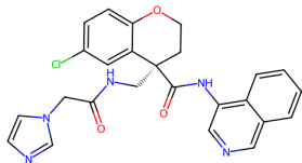
7GJ2, QH6 (5.54)
