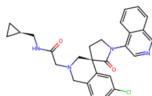
7GNK, SOX (7.08)
