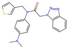
7GD5, M0X (5.75)
