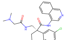
7GJO, QH6 (5.3)
