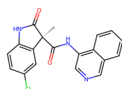
7GK1, QSF (5.22)
