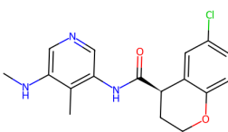
7CKZ, R2L (4.49)
