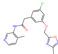
7GFG, OAO (4.62)
