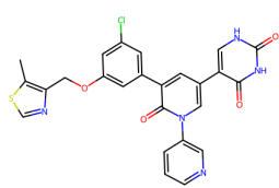
7N44, O6I (7.38)
