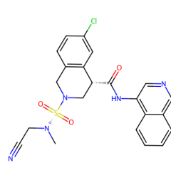
7GLG, R95 (6.93)
