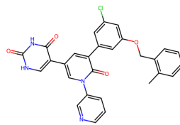
7MBN, Y5P (7.0)
