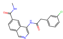
7CMM, RL8 (6.05)
