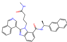
7UR9, O5F (7.74)
