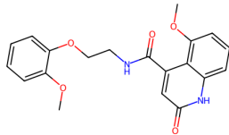
7GE1, N43 (5.69)
