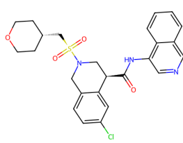
7GLL, RAQ (6.82)
