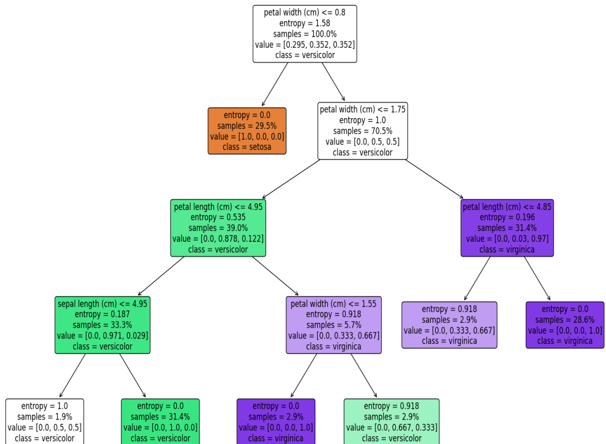
Decision Tree for Iris Dataset
