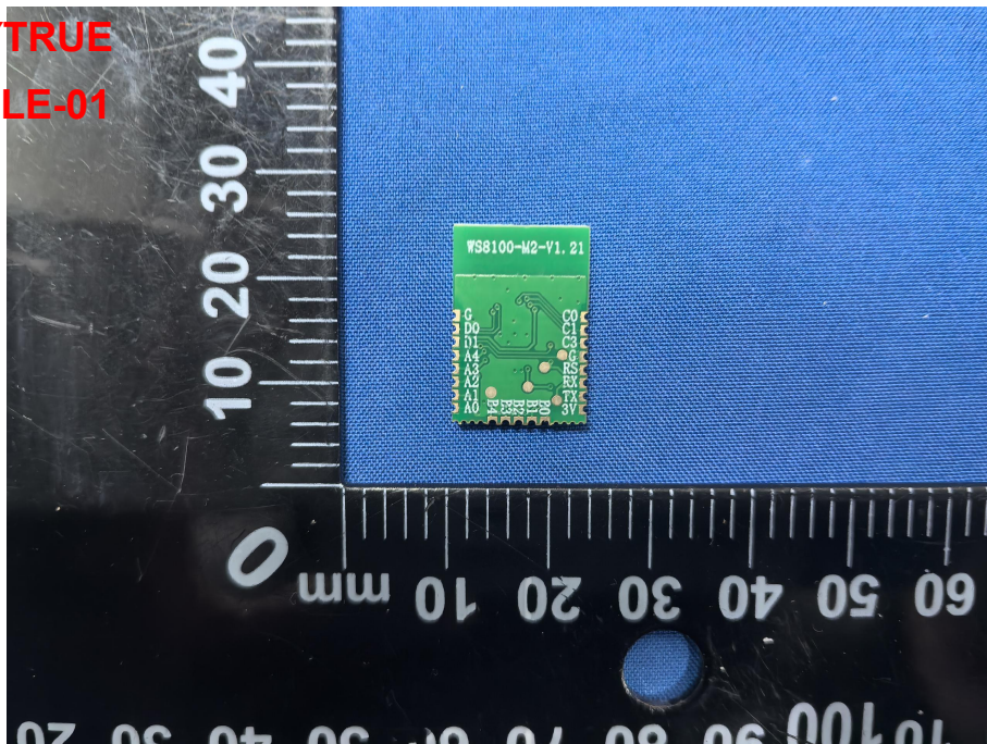
Model: SDC-LE-01 Photo 3
