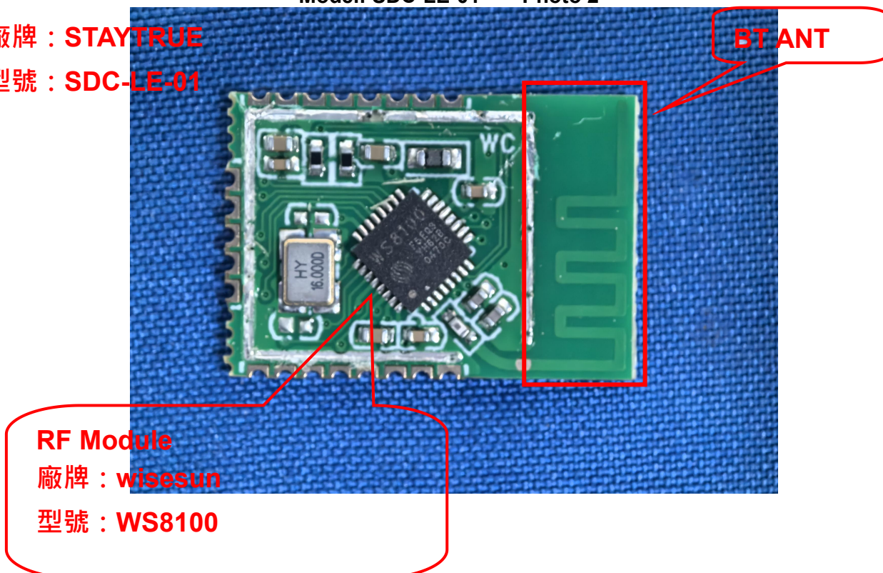
Model: SDC-LE-01 Photo 2
