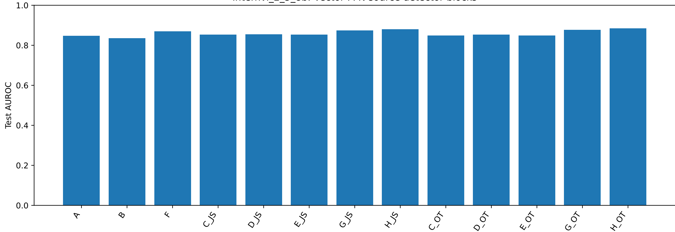
internvl_2_5_8b: Vector FFN source detector blocks
