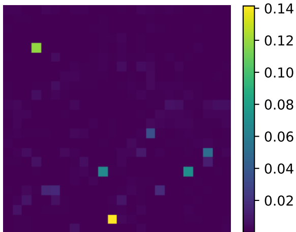
HALL T
