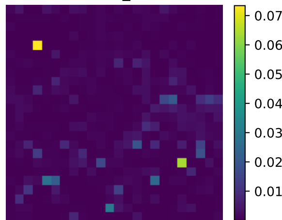
HALL P_FFN
