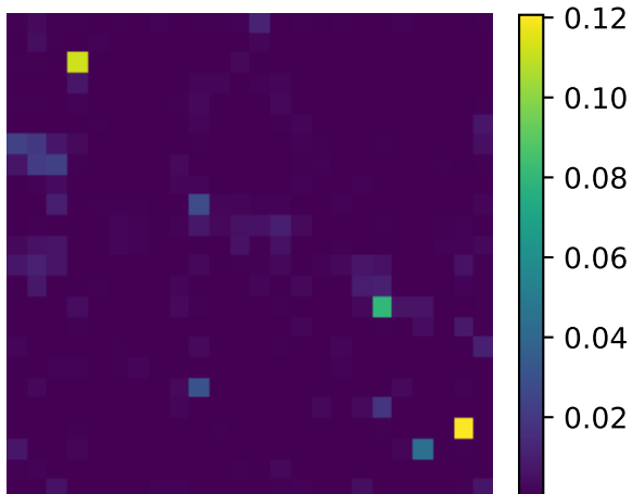
REAL T
