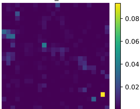
REAL P_WRITE
