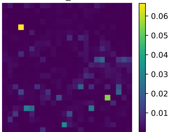
HALL P_WRITE
