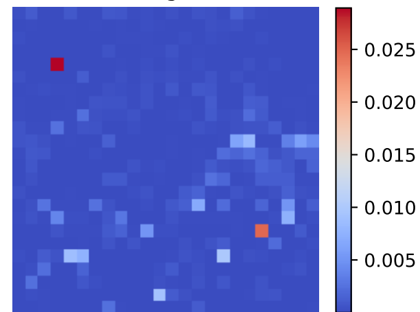
HALL signed-Q
