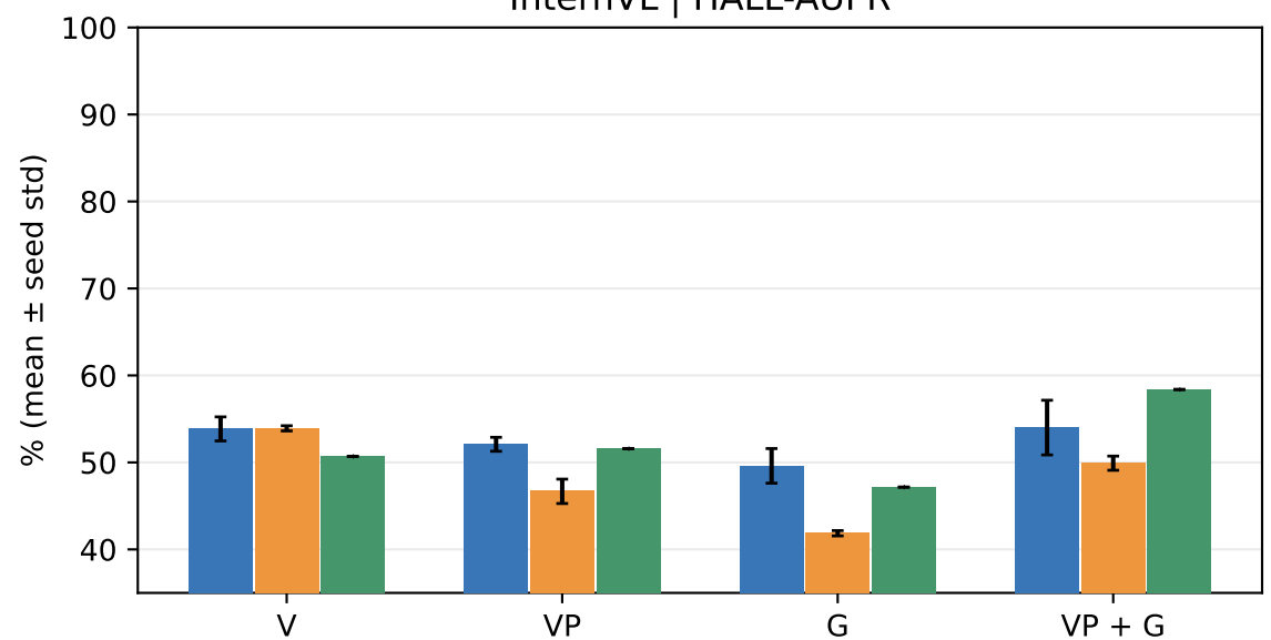
InternVL | HALL-AUPR
