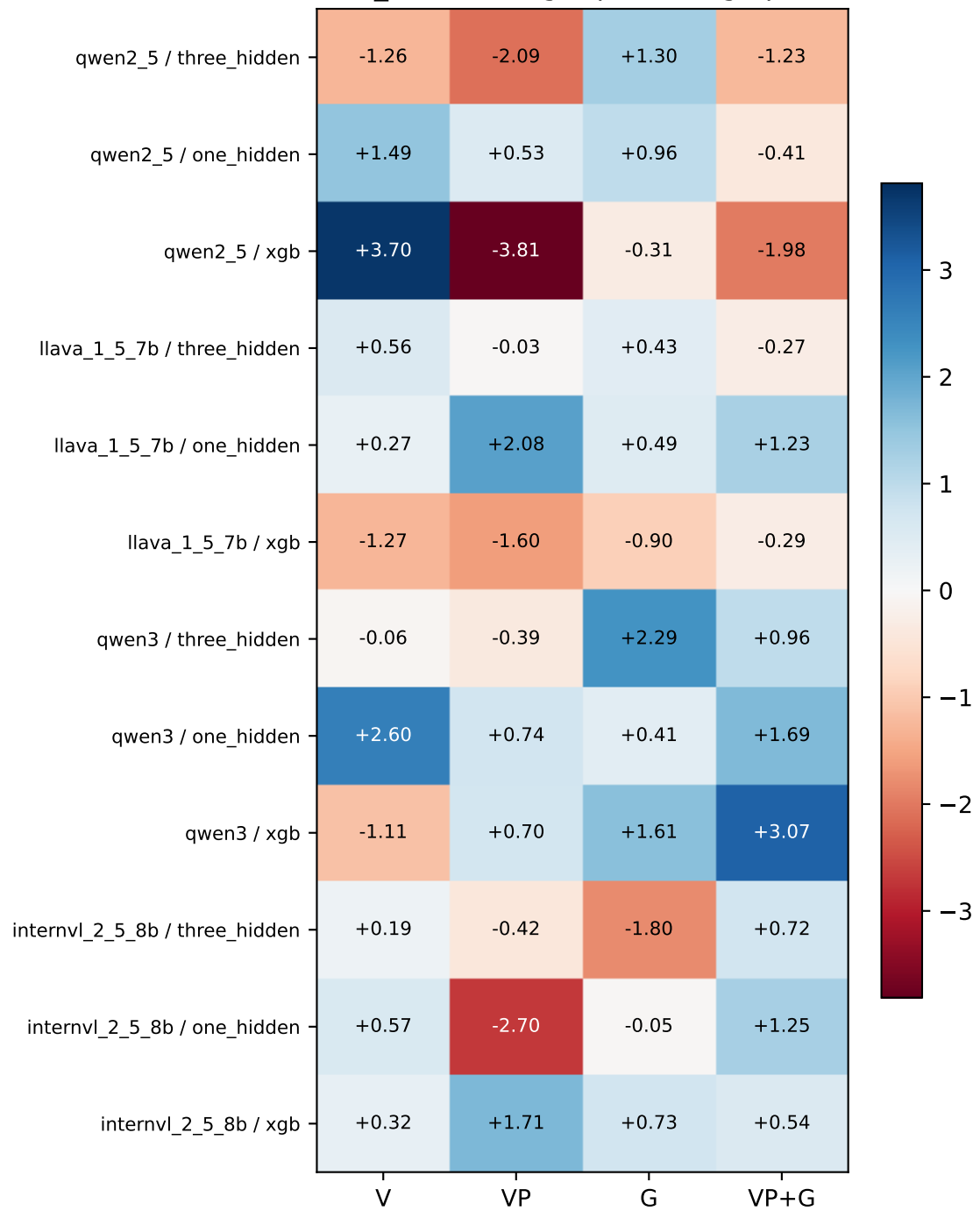
HALL_AUPR change (percentage points)
