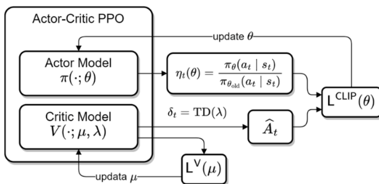
图 6: Actor 出动作、Critic 打分并回传梯度指导 Actor
