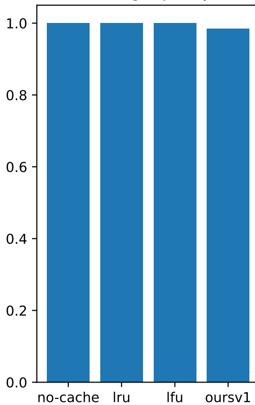
average quality
