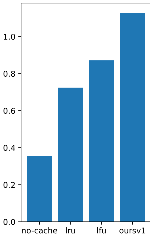
average throughput(req/s)
