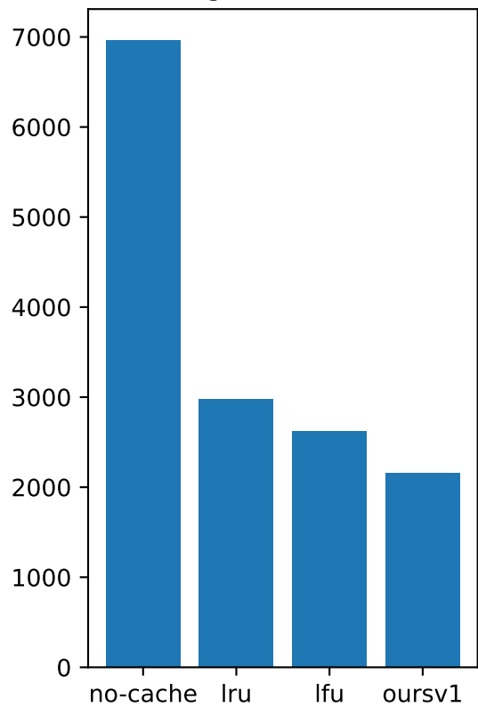
average TTFT(second)
