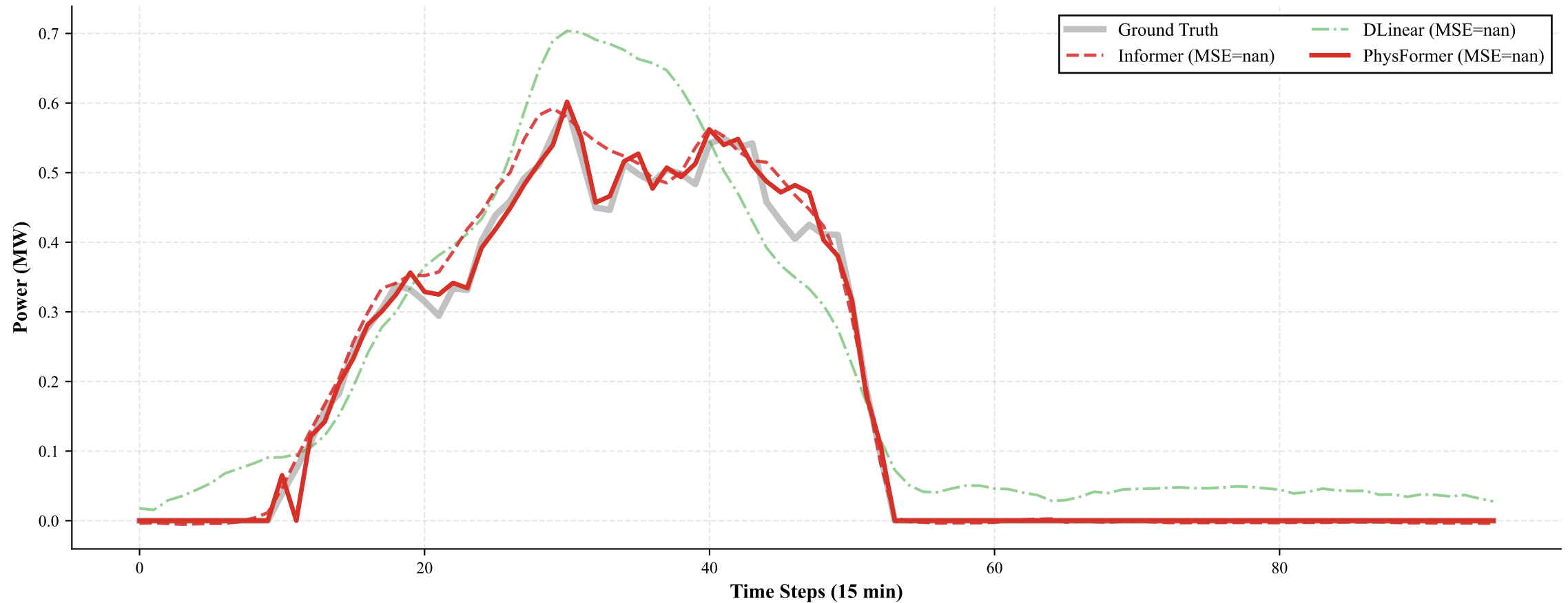
Multi-Model Forecasting Comparison — PV Channel
