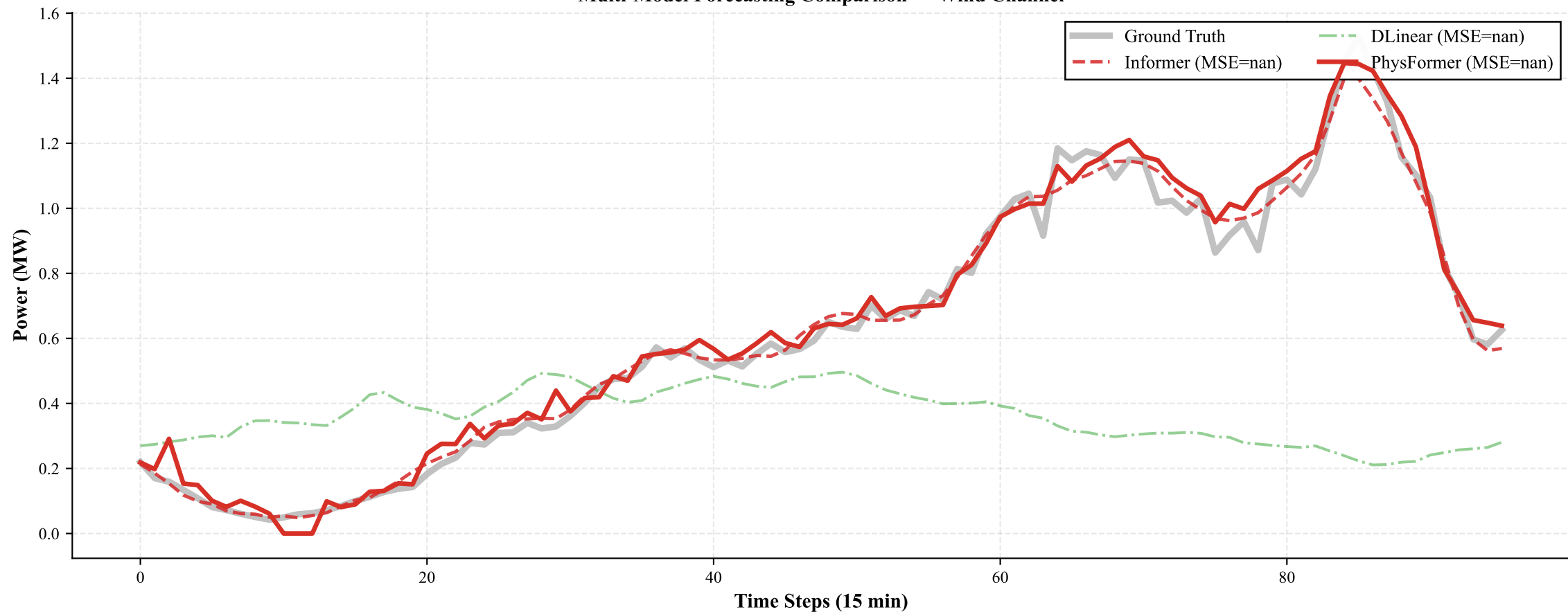
Multi-Model Forecasting Comparison — Wind Channel
