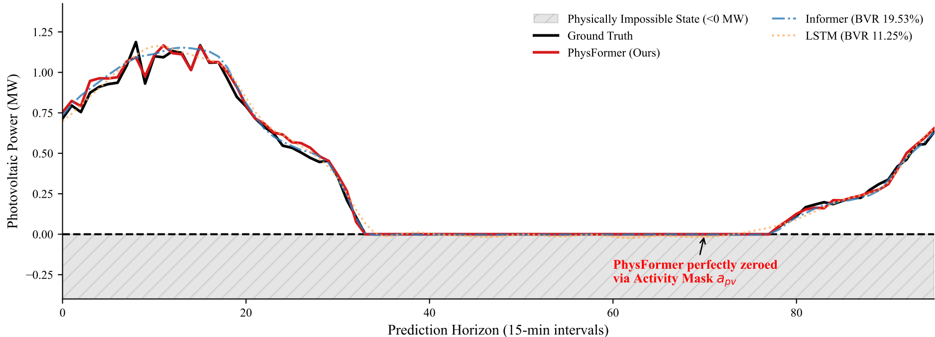
Fig. 6: Night-time PV Boundary Adherence Evaluation
