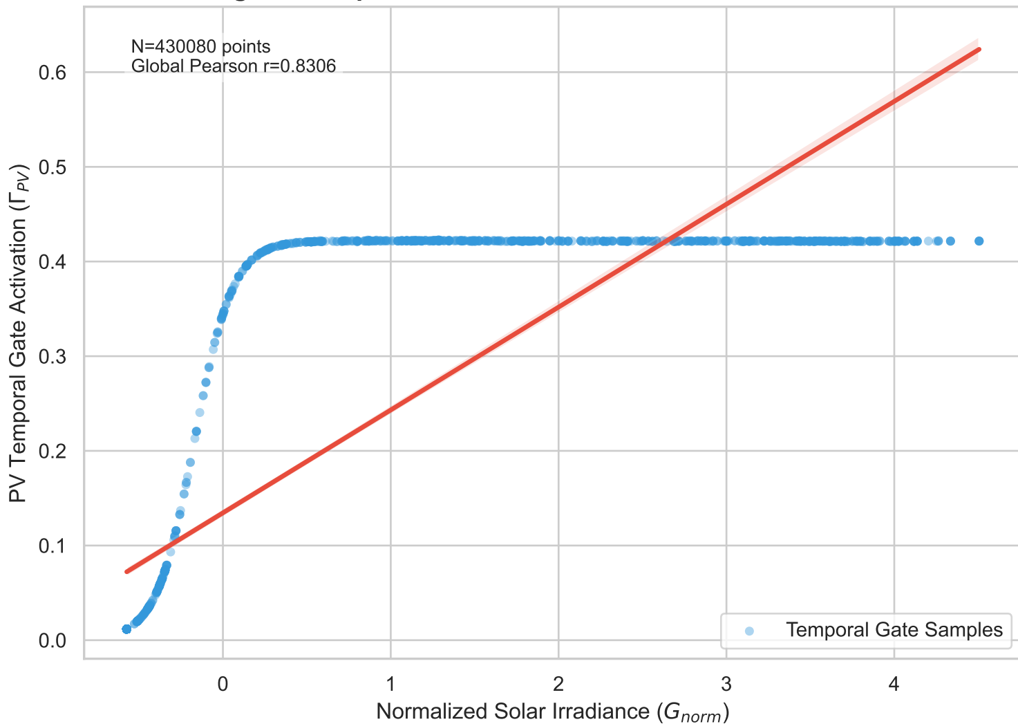
Figure 3: Imprinted Gate-Irradiance Correlation in PGCC
