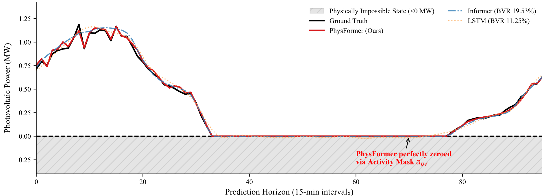
Fig. 6: Night-time PV Boundary Adherence Evaluation
