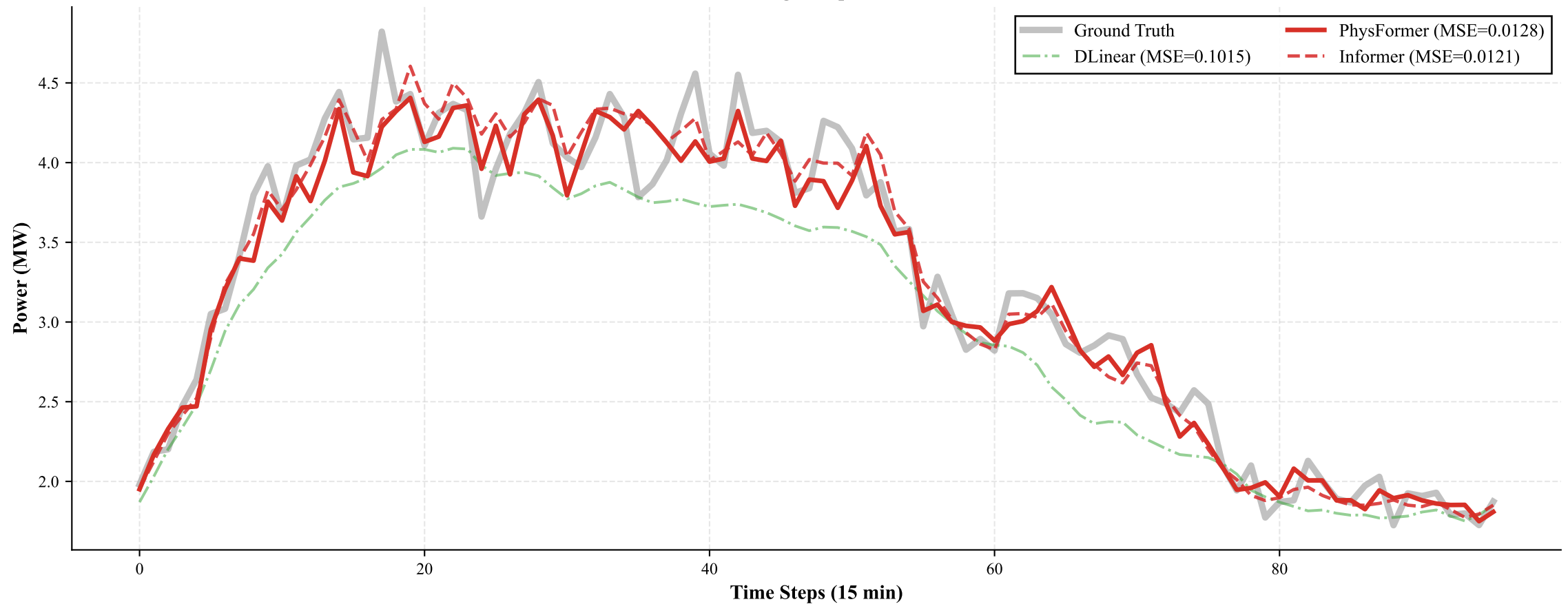
Multi-Model Forecasting Comparison — Load Channel
