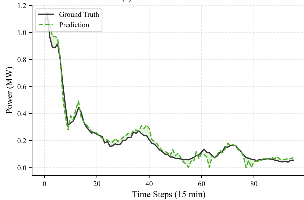
(c) Wind Power Forecast
