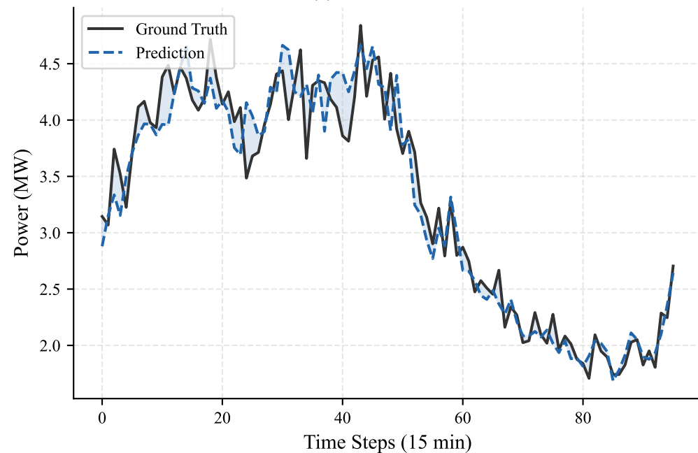
(a) Load Forecast
