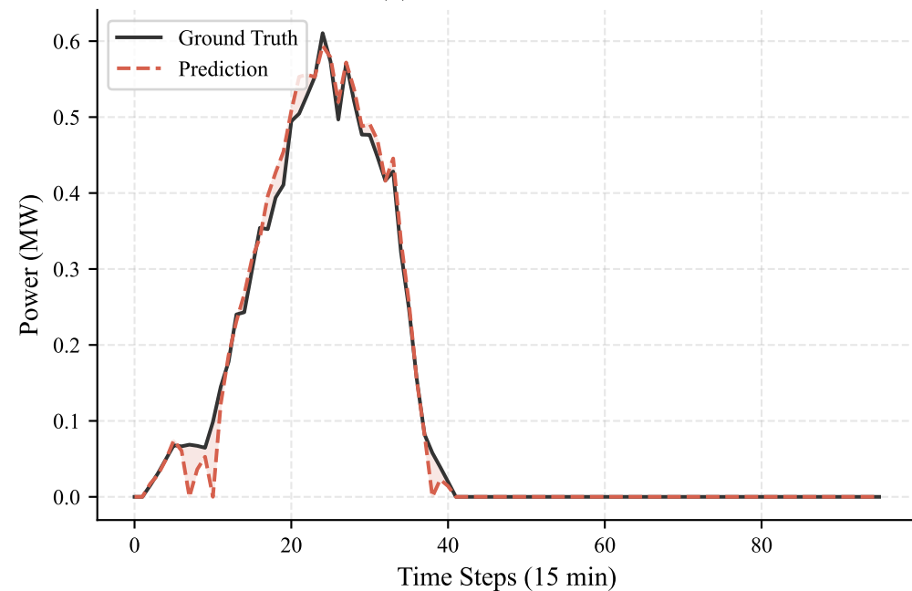
(b) PV Power Forecast
