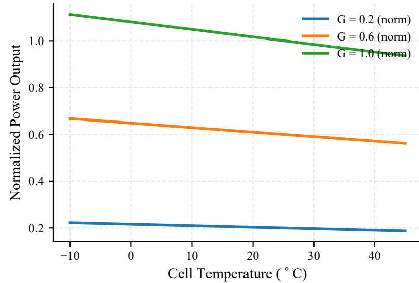
(a) PV Temperature Degradation
