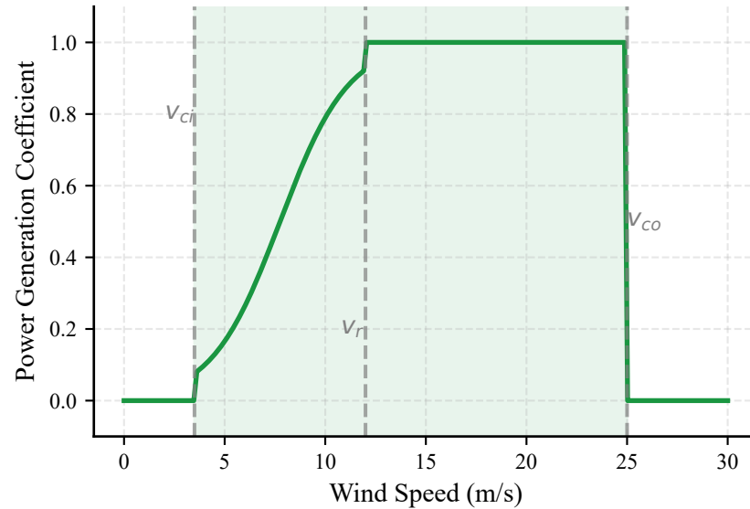
(b) Wind Turbine Power Curve
