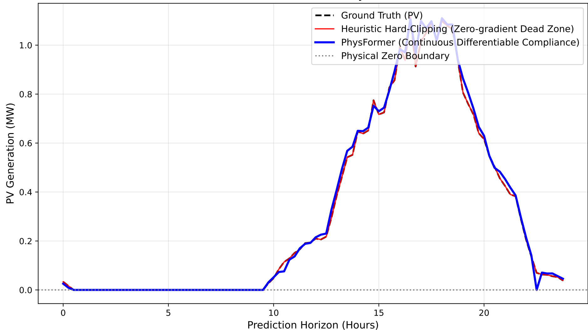
Non-differentiable Dead Zone vs. Structural Physical Manifold (PV Generation)
