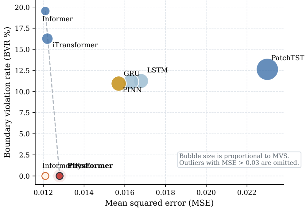
Figure 5: PhysFormer combines zero boundary violations with accuracy close to the strongest unconstrained baselines. High-error outliers with MSE > 0.03 are omitted.
