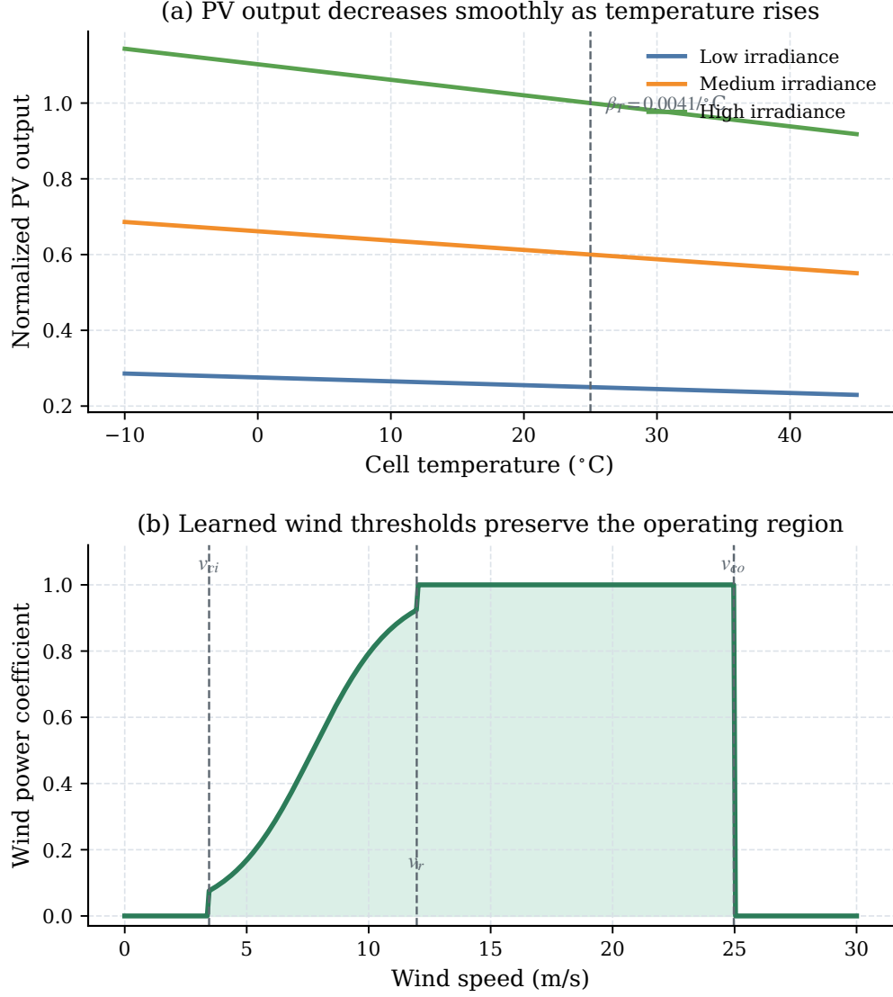
Figure 2: The learned PV and wind mappings preserve physically meaningful monotonicity and operating thresholds. The PV branch maintains smooth temperature degradation, while the wind branch retains the cut-in, rated, and cut-out structure reported in Table 5.
