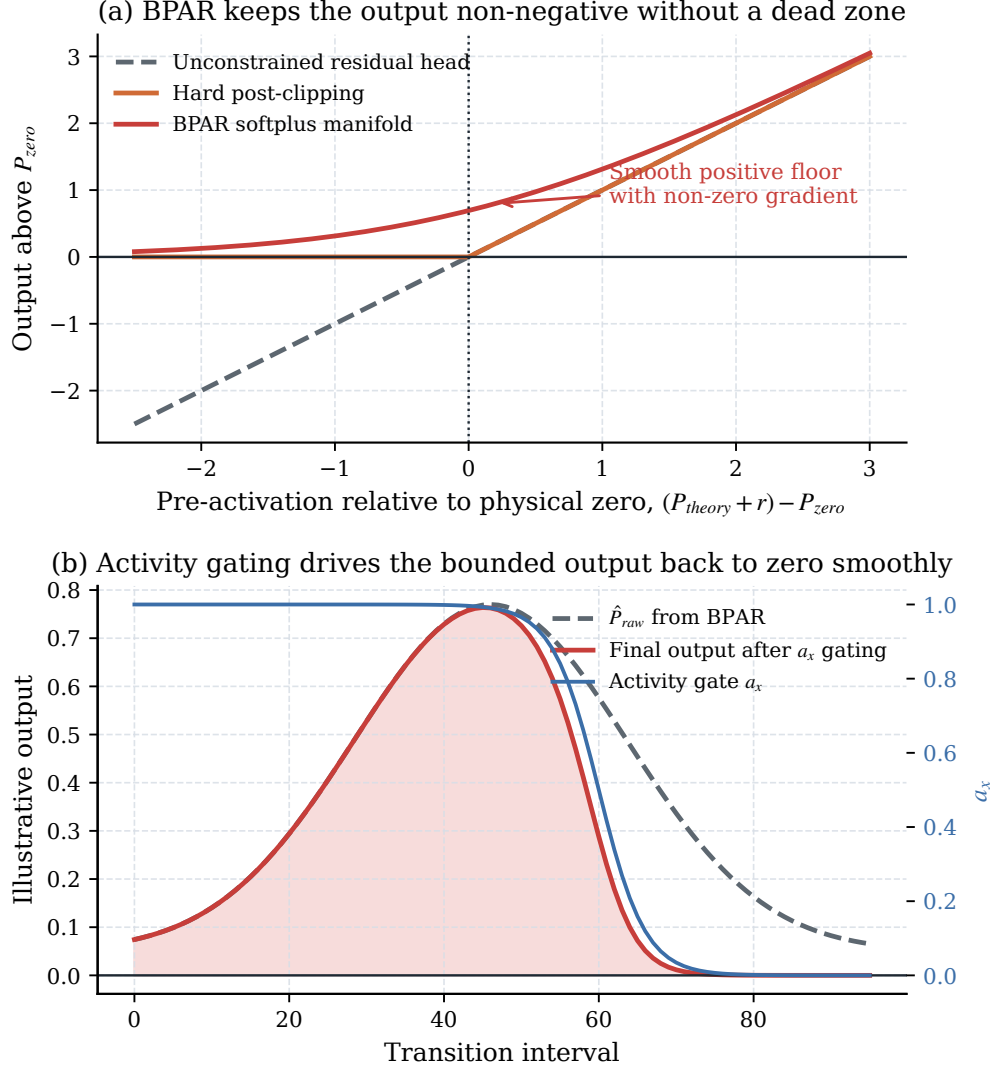
Figure 3: BPAR removes the hard dead zone of post-clipping and, together with activity gating, smoothly pulls the forecast back toward the physical zero boundary. Panel (b) is an illustrative mechanism plot under the adopted normalization setting.
