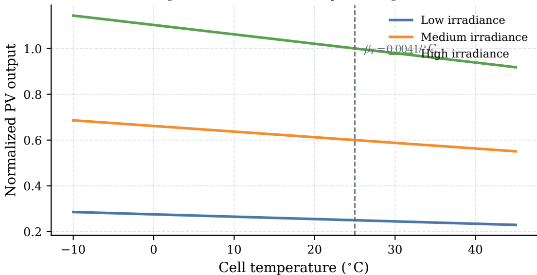
(a) PV output decreases smoothly as temperature rises
