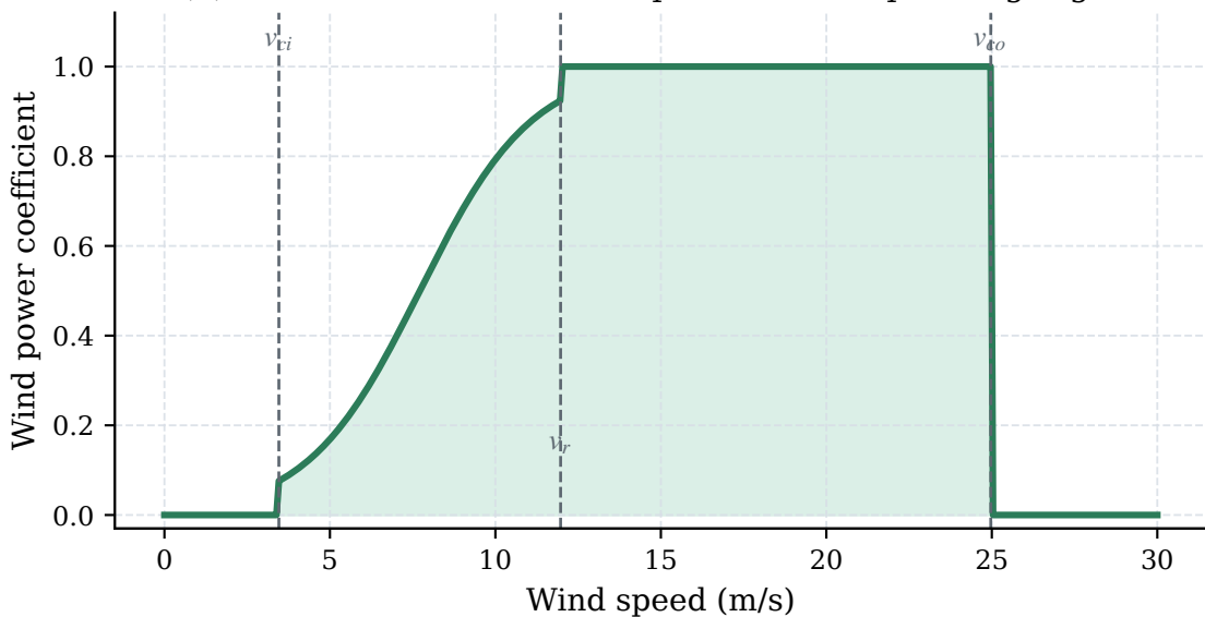
(b) Learned wind thresholds preserve the operating region
