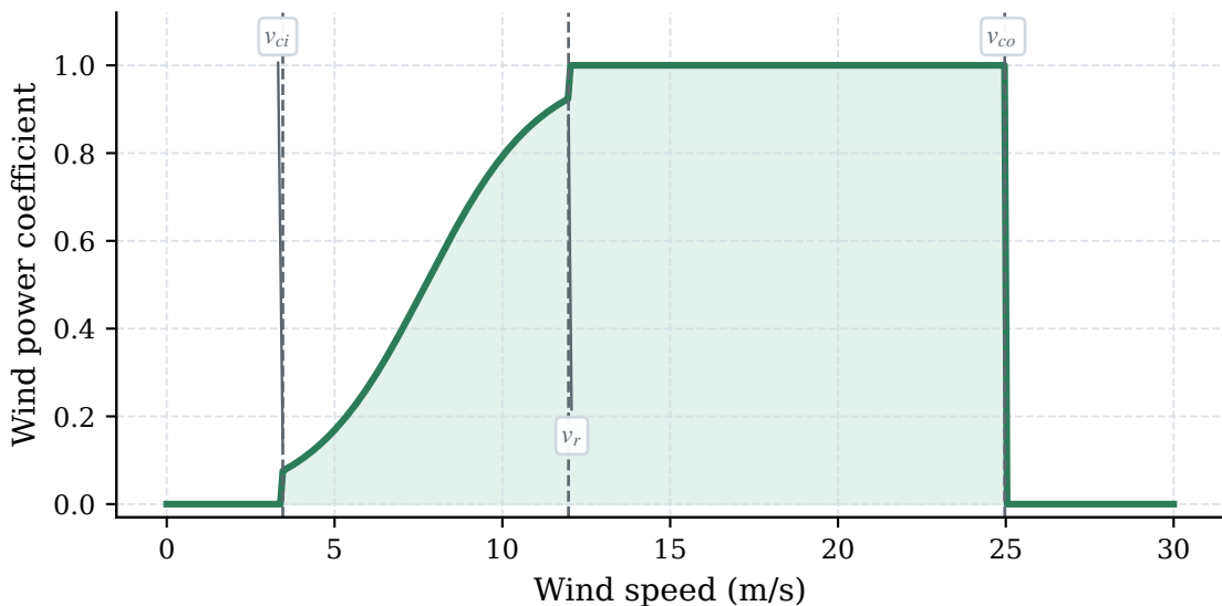
(b) Learned wind thresholds preserve the operating region
