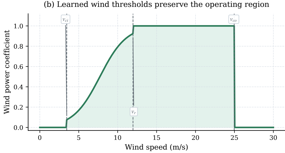
Figure 2: The learned PV and wind mappings preserve physically meaningful monotonicity and operating thresholds. The PV branch maintains smooth temperature degradation, while the wind branch retains the cut-in, rated, and cut-out structure reported in Table 5.
