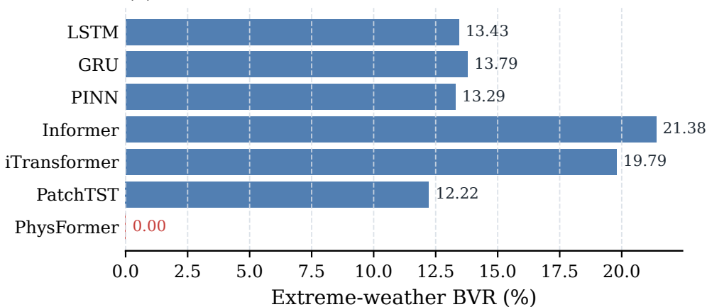
(b) Extreme-weather BVR
