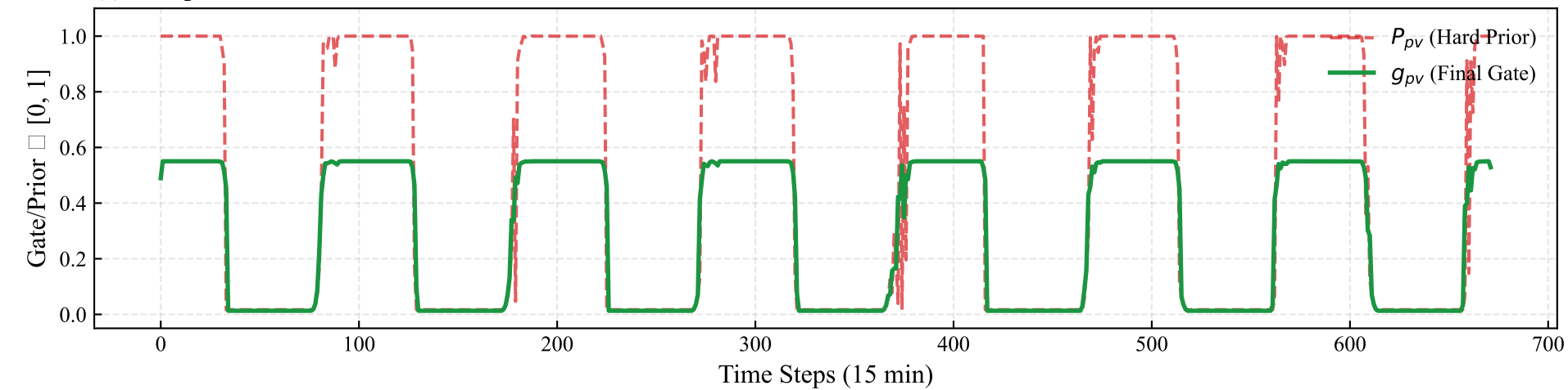
(c) Comparison: Final Gate vs Hard Prior
