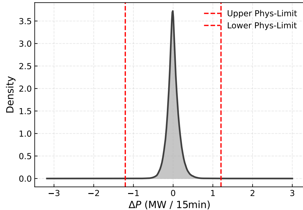
(a) Load Ramp Rate Violations: 0.05%
