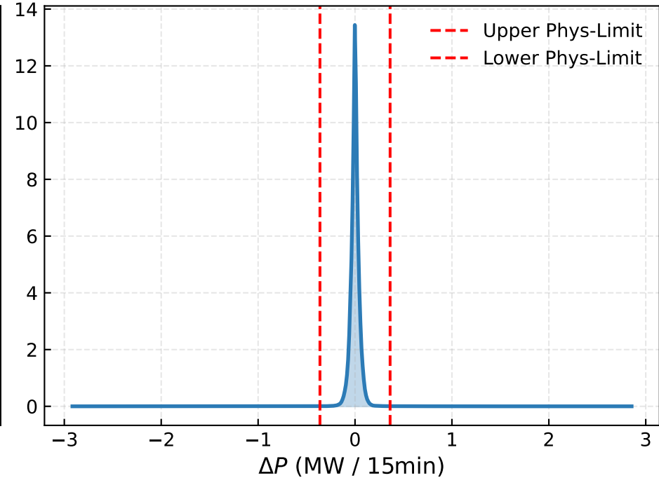
(c) Wind Ramp Rate Violations: 0.47%
