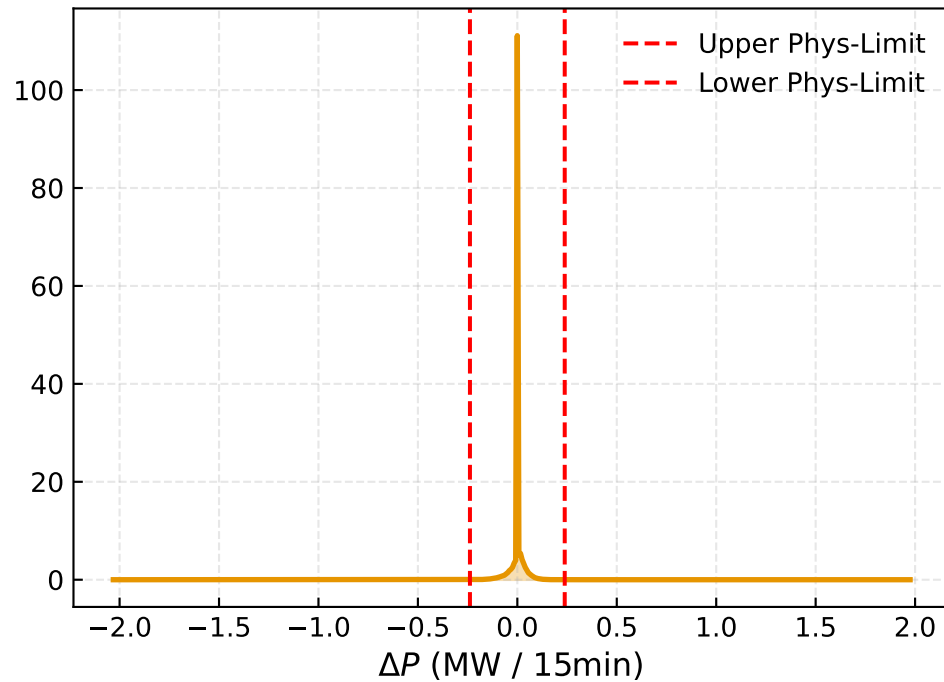
(b) PV Ramp Rate Violations: 0.13%
