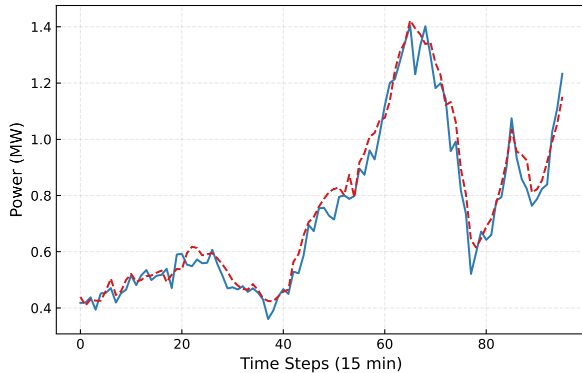
(c) Wind Power Forecast
