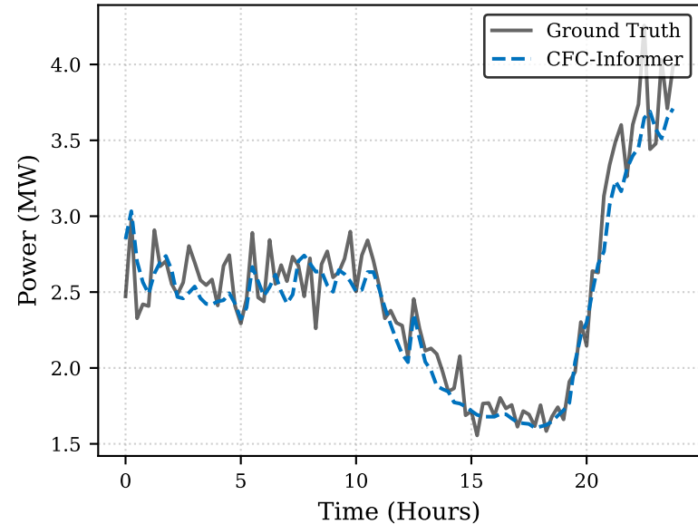
(a) Load Forecasting (MAE=0.141)
