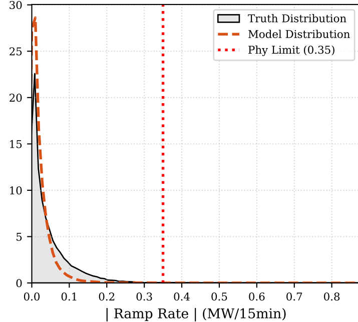
(c) Wind Dynamics Violation Rate: 0.44%
