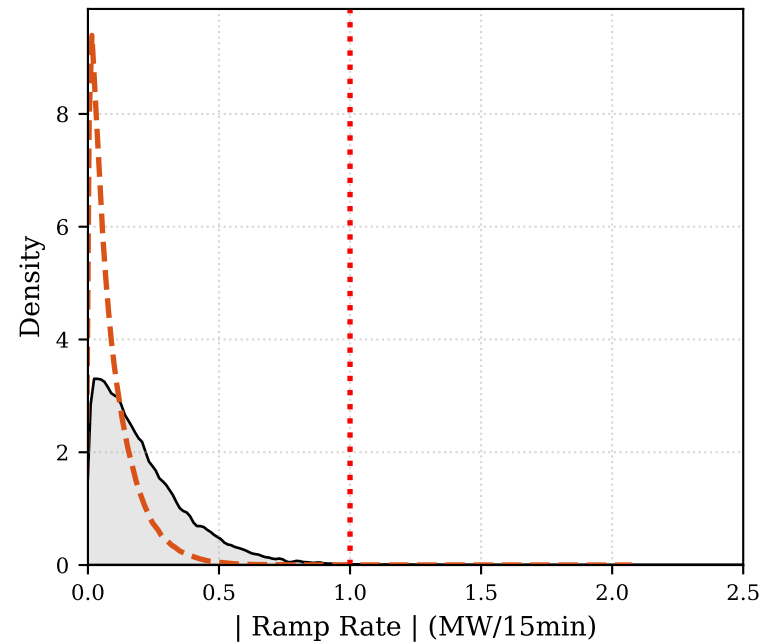
(a) Load Dynamics Violation Rate: 0.06%
