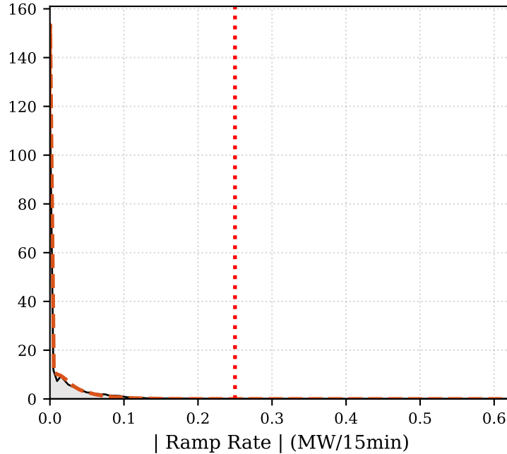
(b) PV Dynamics Violation Rate: 0.10%
