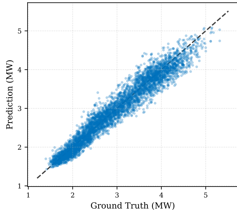
(a) Load Regression ( R^2=0.947 )
