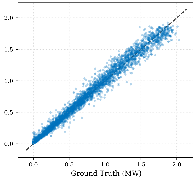
(c) Wind Regression ( R^2=0.986 )
