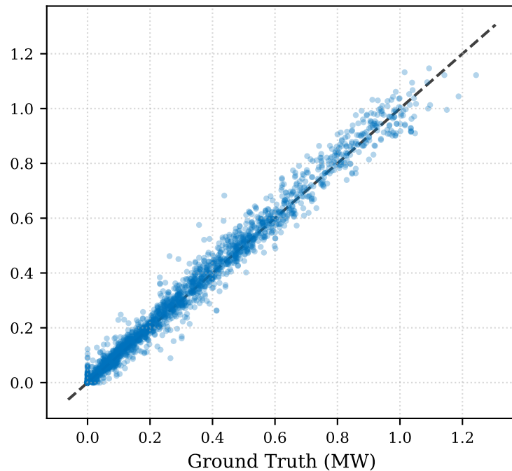
(b) PV Regression ( R^2=0.989 )
