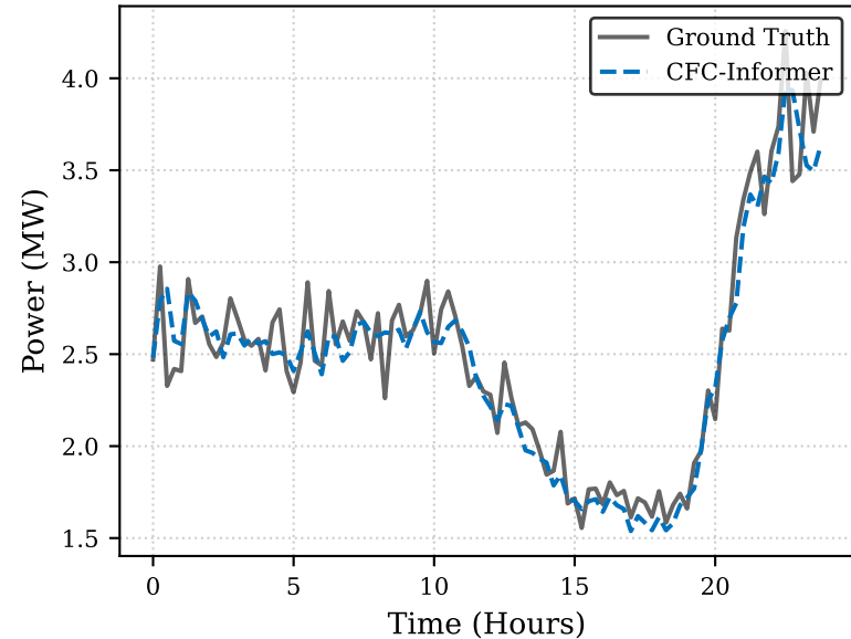
(a) Load Forecasting (MAE=0.127)
