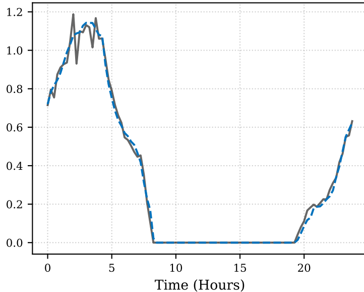
(b) PV Forecasting (MAE=0.017)
