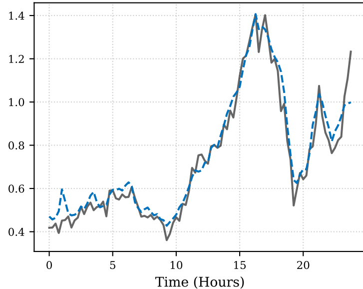
(c) Wind Forecasting (MAE=0.043)
