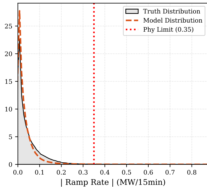
(c) Wind Dynamics Violation Rate: 0.61%
