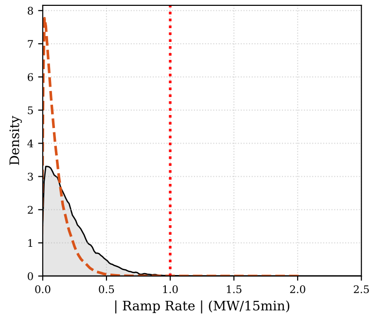
(a) Load Dynamics Violation Rate: 0.05%
