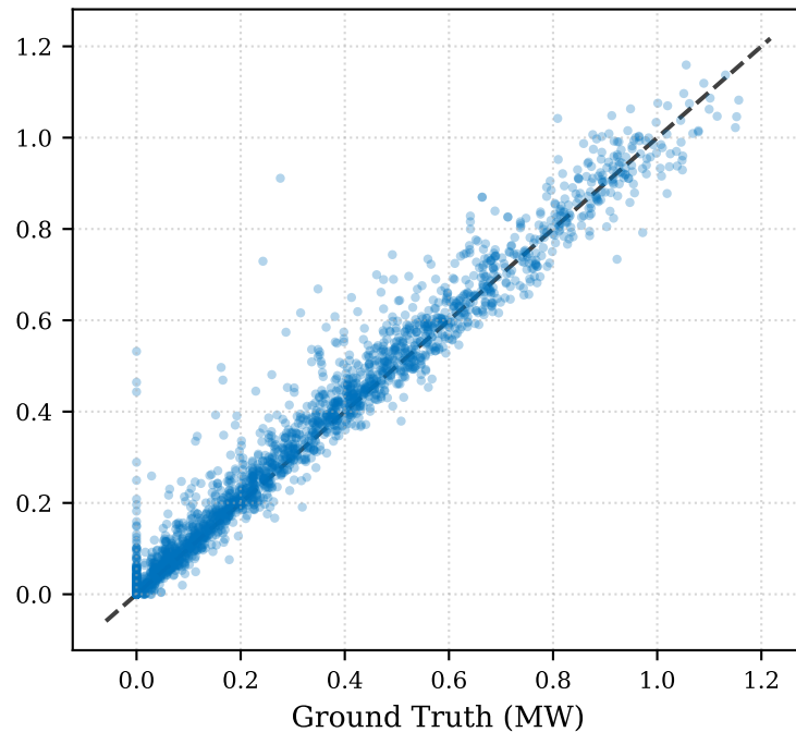
(b) PV Regression ( R^2=0.975 )
