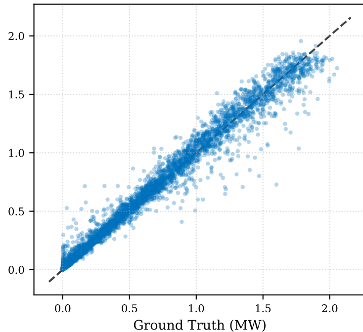
(c) Wind Regression ( R^2=0.977 )
