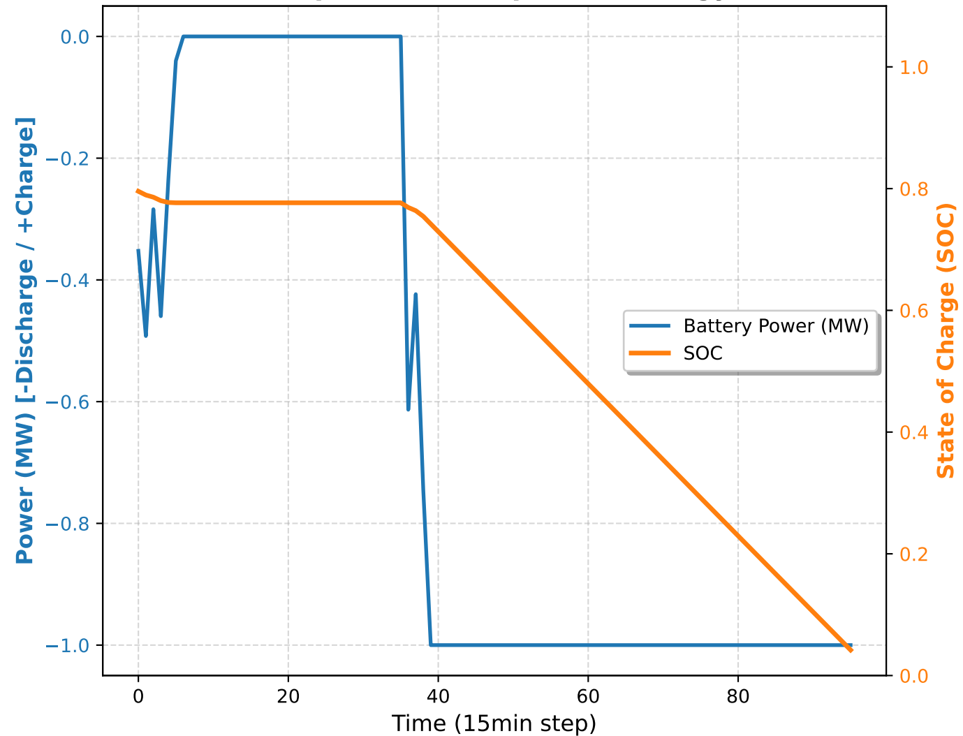
Adaptive VPP Dispatch Strategy
