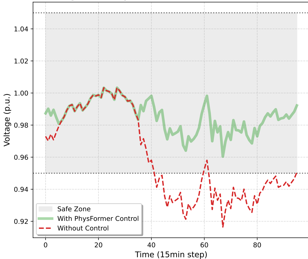
Voltage Stability at Node 32 (Stress Factor=1.0x)
